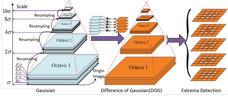
Figure 4.3: Scale-space extrema detection ( https://blog.csdn.net/lhanchao/article/details/52345845 )
