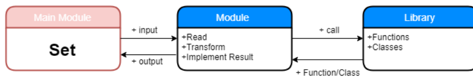
Figure 3.4: Library process
