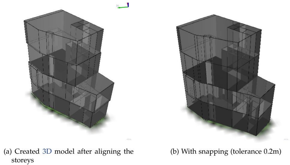
Figure 6.21.: Comparison of 3D storey alignment results with and without snapping
