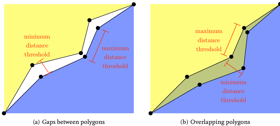
Figure 2: Defining a threshold for vertex and edge snapping. The threshold to use should be larger than the largest minimum distance between the matching boundaries, and smaller than the minimum distance between vertices of a single polygon.
