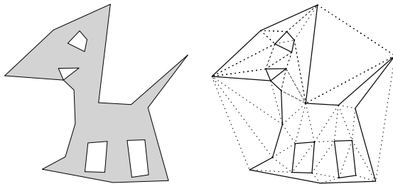
Figure 7: (a) A polygon with 4 holes. (b) The constrained triangulation of the segments of this polygon.
