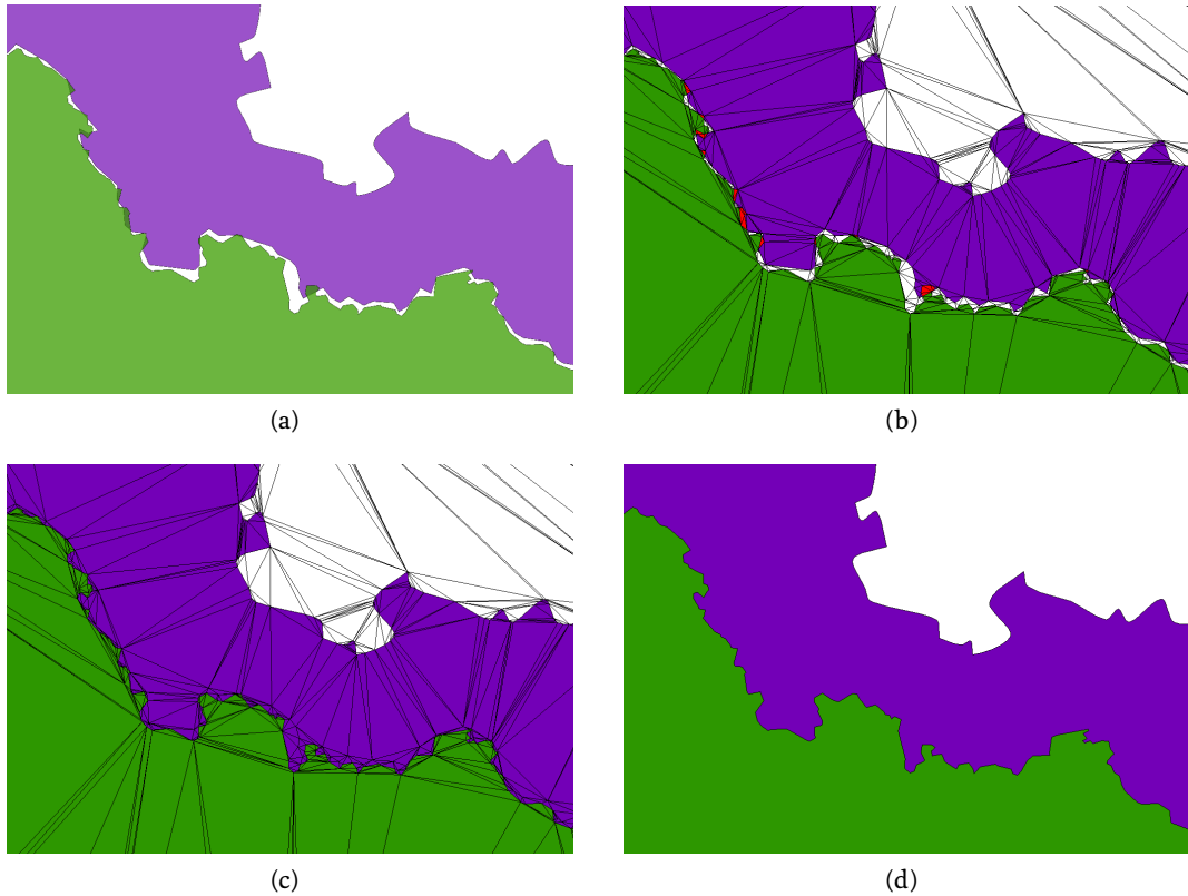
Figure 6: (a) Original dataset with two polygons. Notice the gaps (white) and the overlaps (darker green). (b) The CT of the input polygons; white triangles have no label, and red ones have > 1 . (c) Triangles are re-tagged such that each triangle has one and only one label. (d) The resulting edge-matched polygons.
