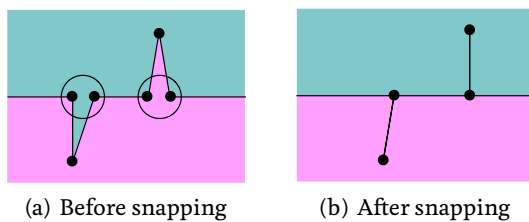
Figure 3: Spikes and punctures can be created by snapping, since the bases of these elongated forms (encircled) might be narrower than the threshold, but their lengths not.
