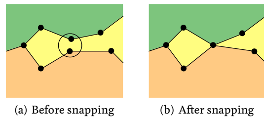
Figure 4: Polygons can be split by snapping, since some parts might be narrower than the threshold (encircled). While this result does not create an invalid result, it can change the number of polygons present and their topological relations, and can therefore be undesirable.
