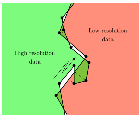
Figure 5: Snapping to the closest line can cause topologically invalid configurations. When two datasets of differing levels of detail are joined together by snapping the vertices of the high resolution dataset to the edges of the low resolution one, a situation where the line reverses on itself is created.
