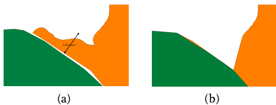
Figure 11: (a) Original dataset, with the tolerance used for snapping. (b) Collapsing of part of a polygon.
