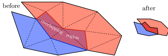
Figure 8: Regions are defined as adjacent triangles with equivalent sets of tags. In this example, the overlapping region between the red and blue polygons is repaired by the tag present along the longest part of the boundary surrounding the region (red).
