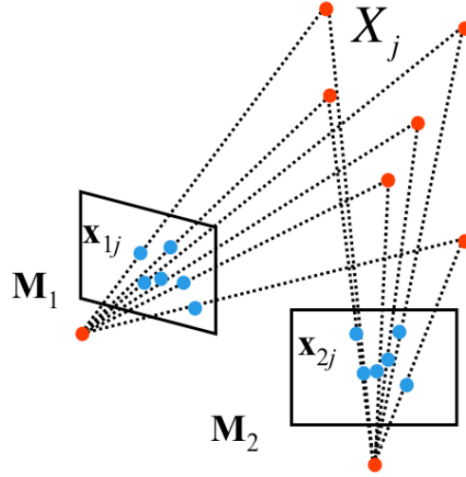
Figure 5: In the algebraic approach, we consider sequential, camera pairs to determine camera matrices M_1 and M_2 up to a perspective transformation. We then find a perspective transformation H such that M_1H = [I \ 0] and M_2H = [A \ B]
