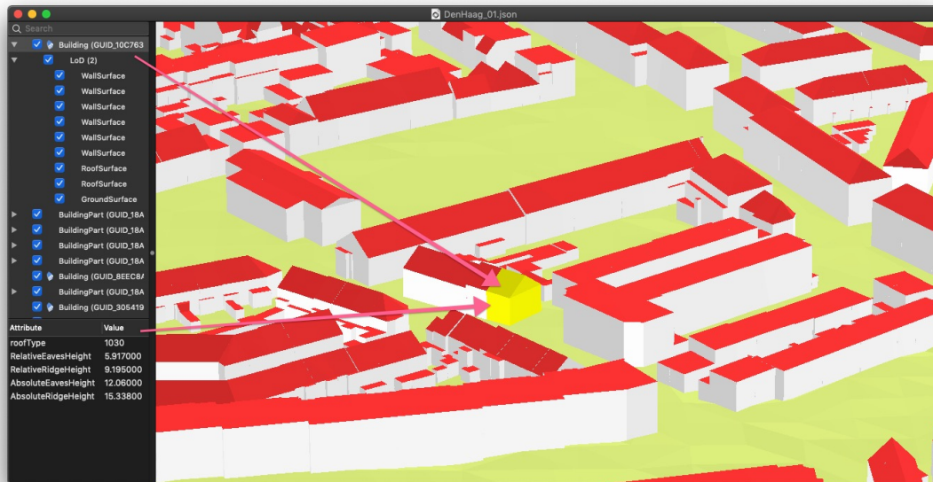
Figure 3: Part of the semantic 3D city model of The Hague, in the Netherlands. Notice that each building is decomposed into its semantic surfaces (wall, roof, and ground) and there are attributes for each. The model is not textured, but semantic models can have textures too.
