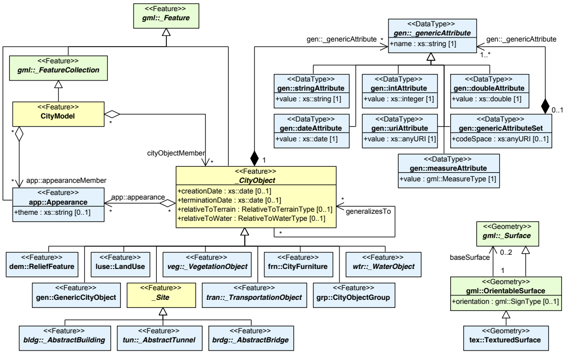
Figure 4: Overview of the UML model for the core of CityGML. (Figure © 2012 Open Geospatial Consortium, Inc.)
