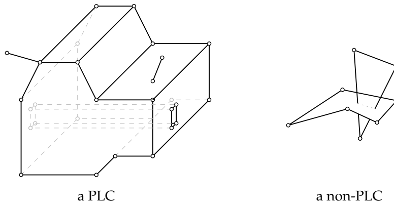
Figure 13: Left: a PLC representing a solid (with a genus of 1) and having one dangling left; notice also that one extra edge is on a polygon. Right: These two polygons do not form a valid PLC because their intersection is not formed of vertices and edges in the PLC.
