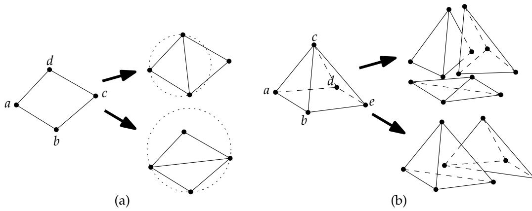
Figure 5: (a) A four-sided convex polygon abcd can be triangulated in two different ways, but the empty circumcircle criterion guarantees that the triangles are as equilateral as possible. Notice that the edge ac is not locally Delaunay, but bd is. (b) In three dimensions, five vertices can be triangulated with either two or three tetrahedra. Although the tetrahedralisation at the bottom has two nicely shaped tetrahedra, they are not Delaunay (the point d is inside the sphere abce , which also implies that b is inside the sphere acde ). The tetrahedralisation at the top respects the Delaunay criterion, but contains one very thin tetrahedron spanned by the points a, b, d and e .
