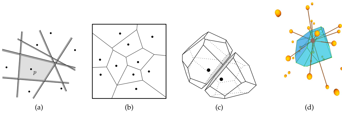
Figure 1: (a) The Voronoi cell \mathcal{V}_p is formed by the intersection of all the half-planes between p and the other points. (b) The VD for a set S of points in the plane (the black points). (c) Two Voronoi cells adjacent to each other in \mathbb{R}^3 , they share the grey face. (d) The Voronoi cell for the red vertex, the red edges are the Delaunay edges that are dual to the Voronoi facets.
