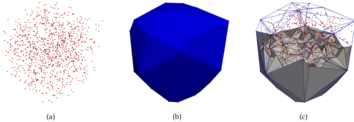
Figure 4: (a) A set of 1000 points randomly distributed in a cube. (b) Its convex hull. (c) The Delaunay tetrahedralisation of the points, 'sliced' in the middle and the upper tetrahedra removed (to be able to visualise the interior).
