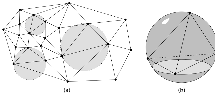
Figure 2: (a) The DT of a set of points in the plane. (b) A Delaunay tetrahedron has an empty circumsphere.
