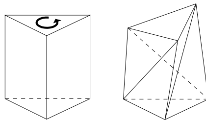
Figure 14: The Schönhardt polyhedron is impossible to tetrahedralise without adding extra vertices inside.
