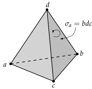
Figure 9: The tetrahedron abcd is correctly oriented since \text{ORIENT}(a, b, c, d) returns a positive result. The arrow indicates the correct orientation for the face \sigma_a , so that \text{ORIENT}(\sigma_a, a) returns a positive result.
