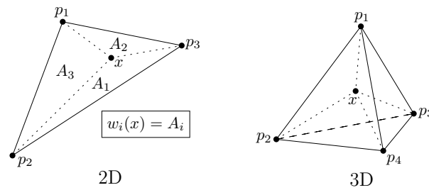
Figure 11: Barycentric coordinates in two and three dimensions. A_i represents the area of the triangle formed by x and one edge.
