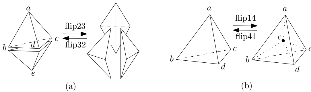
Figure 8: The 4 different kinds of flips in 3D.
